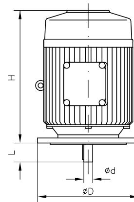
Motor design B 5 (V1)
